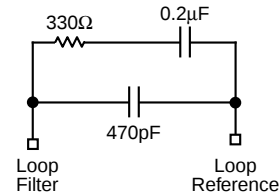
Figure 1. External Loop Filter Connection
